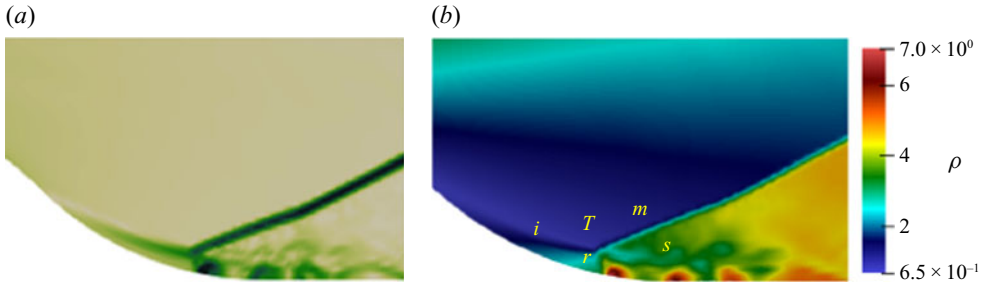
Figure 20. (a) Zoomed-in view of stationary shock wave for M_s = 3.8 . Numerical schlieren (b) density contours with incident shock wave ( i ), reflected shock wave ( r ), Mach stem ( m ), slip line ( s ) and TP ( T ).
