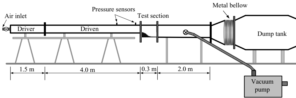
Figure 1. Schematic of the shock-tube facility.
