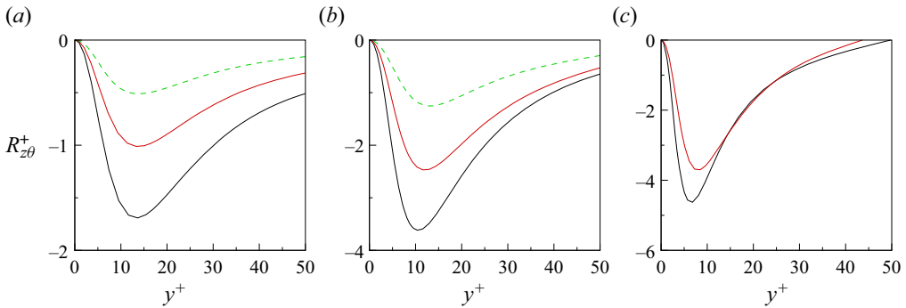
Figure 8. Radial distributions of R_{z\theta}^+ = \overline{wv}^+ in inner coordinates: black solid line indicates Ta = 5000 ; red solid line indicates Ta = 3000 ; green dashed line indicates Ta = 1500 . Plots for (a) Re = 5765 , (b) Re = 1825 , (c) Re = 600 .
