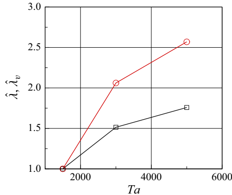
Figure 12. Plots of \hat{\lambda} = \lambda/\lambda_P , \hat{\lambda}_v = \lambda_v/\lambda_P ratios versus Taylor number at Re = 600 : red circles indicate \hat{\lambda} ; black squares indicate \hat{\lambda}_v .
