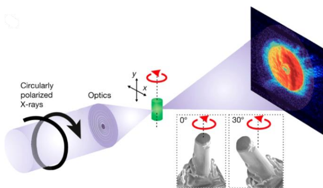
Figure 1. Schematic of magnetic tomography setup. Ptychographic scans are performed with circularly polarized X-rays incident on the sample, which is rotated around the y-axis. To access all three components of the magnetization, tomographic data is collected for two sample orientations, as shown in the inset. Reproduced with permission from [7].
