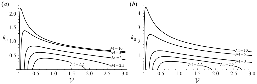
Figure 6. Critical wavenumber k_c (a) and cut-off wavenumber k_0 (b) versus \mathcal{V} for a range of values of \mathcal{M} .
