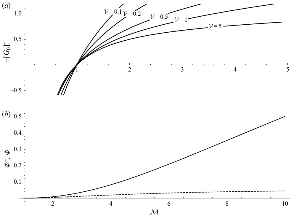
Figure 4. (a) The jump in pressure gradient -[G_0]^\pm across the intrusion front versus the viscosity ratio for various values of \nu . (b) The rate of work done in deforming the upper surface just to the left (dashed) and right (solid) of the intrusion front as a function of \mathcal{M} for \nu = 1 .
