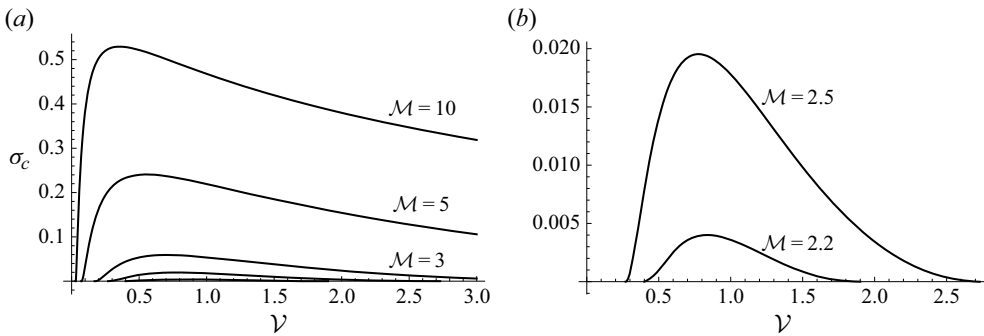
Figure 10. Critical growth rate \sigma_c versus \mathcal{V} for a range of values of \mathcal{M} .
