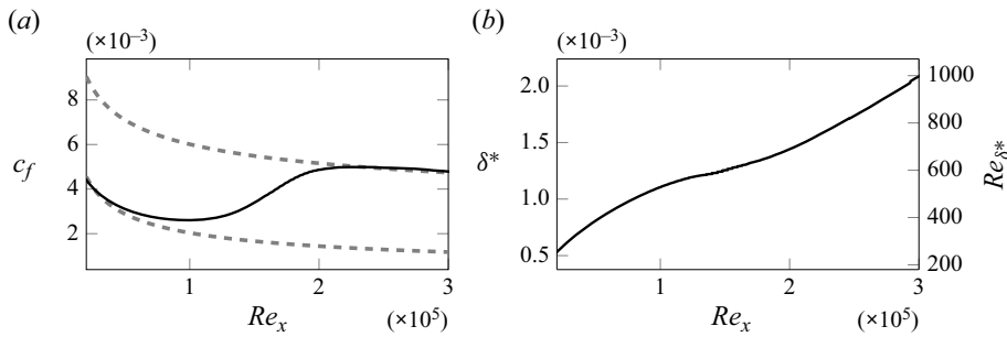
Figure 1. (a) Skin friction coefficient. The dashed lines represent the values for laminar and turbulent boundary layer, and are included for comparison. (b) Evolution of the displacement thickness \delta^* .
