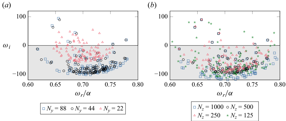
Figure 25. Mesh convergence study for the eigenvalue solver, showing the spectrum for different mesh sizes. (a) Number of wall-normal points varied for a fixed N_z = 500 . (b) Number of span points for a fixed N_y = 44 .
