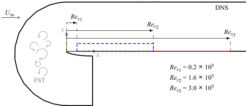
Figure 2. Two-dimensional diagram of the computational set-up. The red line and blue rectangle respectively indicate the surface and volumetric domain extracted from the snapshots to be used in the present work.
