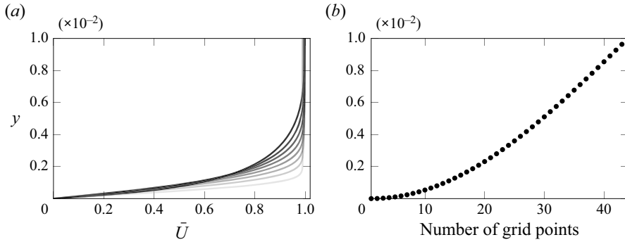
Figure 3. (a) Mean streamwise velocity profiles at Re_x = [0.2 : 0.2 : 1.6] \times 10^5 , from light to dark. (b) Wall normal distribution of the discretisation used for stability analysis.
