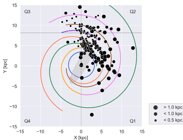
Figure 3. HMSFR distribution in the Milky Way based on maser parallaxes, shown in a plan-view of the Milky Way seen from the north Galactic pole. Data used are from Reid et al. (2019); VERA Collaboration et al. (2020); Xu et al. (2021); Hyland et al. (2022b), and references therein. Adapted figure from Immer and Rygl (2022).
