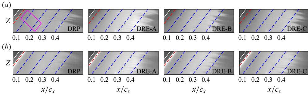
Figure 13. Transition front visualisation at \alpha = 2.5^\circ and Re = 2.5 \times 10^6 for (a) plasma-off and (b) plasma-on. Flow comes from the left and measurements are taken for DRP, DRE-A, DRE-B and DRE-C (columns from left to right).
