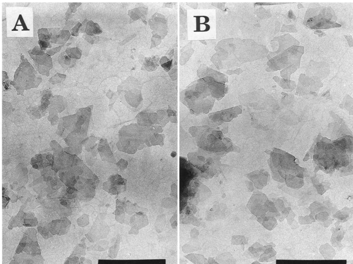
Figure 6. TEM micrographs of I/S showing the appearance of linear edges bounded by 60^\circ and 120^\circ angles at particle boundaries and within aggregates. The regularity of these angles results from crystal growth processes within aggregates. Both A) and B) are 71% expandable I/S. Scale bar is 1\ \mu\text{m} .
