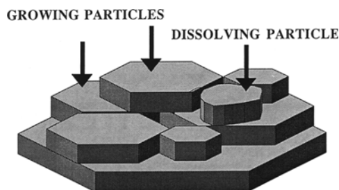
Figure 10. Sketch of I/S aggregate made up of smectite layers, illite layers, and two-layer hybrid particles. Euhedral particles represent growing illite layers, rounded particles represent dissolving smectite or illite.
