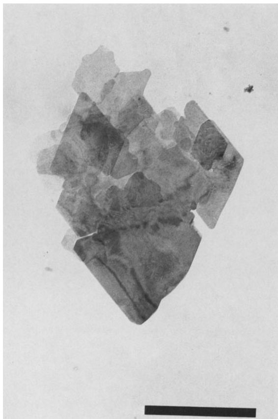
Figure 7. A coalescent particle of 10% expandable I/S showing both rounded (dissolving) and euhedral (crystallizing) particles within the aggregate. The overall shape of the aggregate approaches a rhombic outline of a large illite particle though it is composed of a mosaic of small particles.
