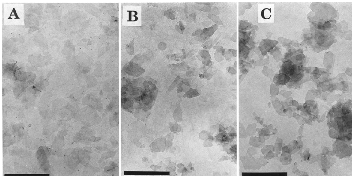
Figure 4. TEM micrographs of I/S run products showing the adhering of individual particles into aggregates. These aggregates were not disrupted by the ultrasonic treatment. A) 100% expandable smectite starting material, B) 71% expandable I/S, C) 42% expandable I/S. Scale bar is 1 \mu\text{m} .
