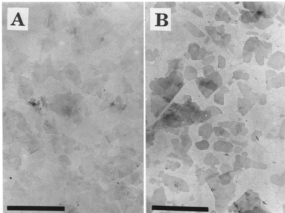
Figure 3. TEM photos showing changes in the degree of rounding during the illitization reaction. The starting smectite (A) has very angular particles, whereas the partly reacted (71% expandable) I/S (B) has more rounded particles, suggesting some dissolution at the edges. Scale bar is 1 \mu\text{m} .
