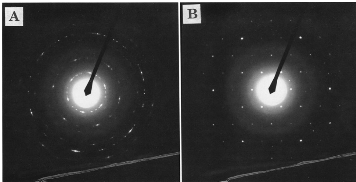
Figure 8. Selected area electron diffraction patterns for A) unreacted smectite (material pictured in Figure 3A) and B) 42% expandable I/S (material pictured in Figure 4C). The streaked spots in the smectite pattern demonstrate that the layers are not completely randomly arranged, but have some coherence of layers in packets. The well-defined spots for the I/S show that a particle of the 42% expandable I/S produces a single crystal diffraction pattern.
