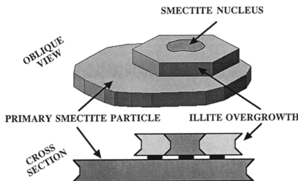
Figure 9. Cartoon representation of a secondary illite layer nucleating on a primary smectite layer. In some cases, small smectite layers may serve as nuclei for illite layer overgrowths.
