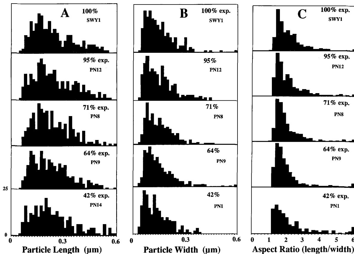
Figure 2. Histogram plots of A) particle length, B) particle width, and C) aspect ratio vs reaction progress. There is no significant change in dimensions of individual particles during the illitization reaction.
