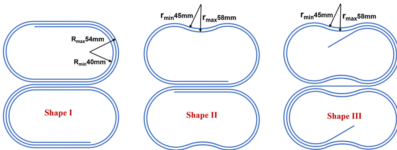
Figure 8. Diagram of the coiling shape for gain fiber.
