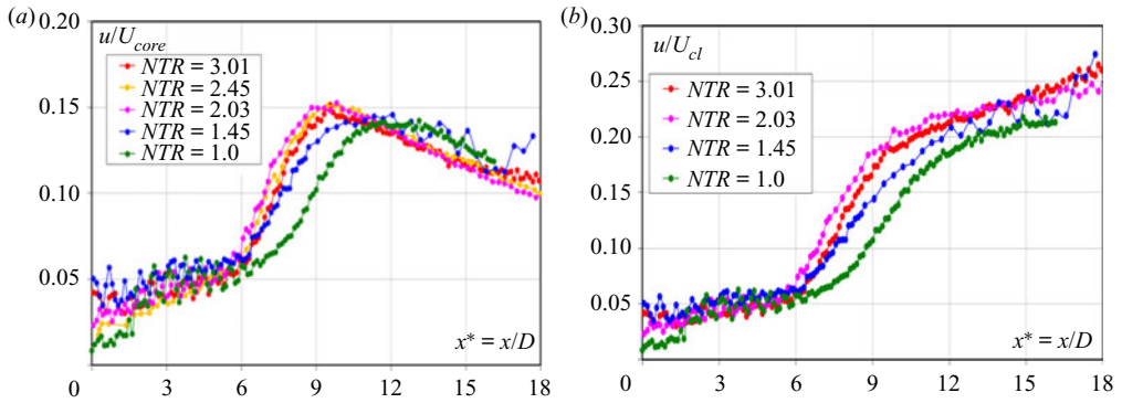
Figure 19. Centreline axial r.m.s. velocity (non-dimensional), NPR = 2.32 for various NTR s Normalising reference velocity; (a) U_{core} , (b) U_{cl} .
