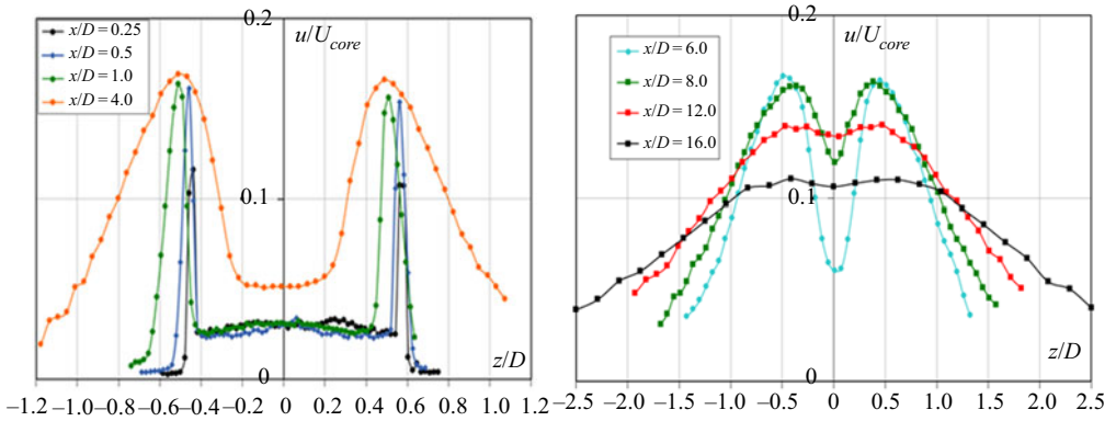
Figure 14. Radial profiles of axial Reynolds stress r.m.s. for NPR = 2.32 , NTR = 2.03 .
