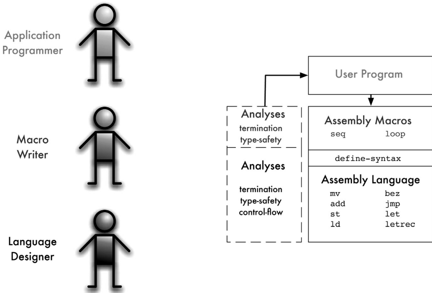
Fig. 1. Workflow to design a language with Ziggurat.
