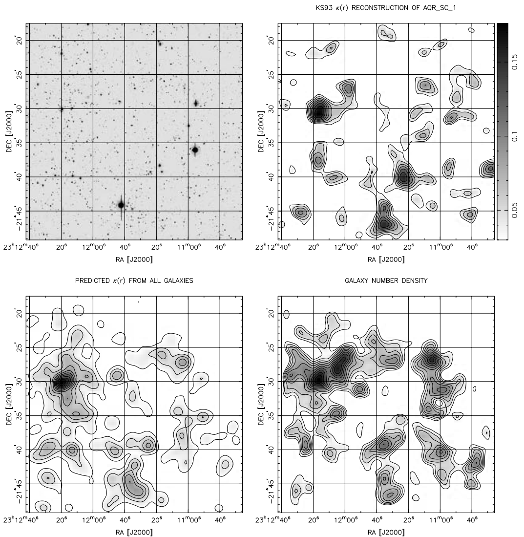
Figure 2. Preliminary results for 1 of the 20 pointings within the Aquarius supercluster region. Top left: R -band image based on ESO WFI imaging. Top right: The surface mass density \kappa_M , determined from weak shear measurements of background galaxies. Bottom left: Predicted surface mass density associated with the light from galaxies in the field, \kappa_L . To generate this plot, the galaxies were all assumed to lie at a single redshift, but in our ongoing analysis we use B – R color information combined with our 2dF spectroscopic redshifts to generate a more accurate measurement of \kappa_L . Bottom right: The number density of all galaxies in the field. Two Abell clusters are located within this field, A2554 ( z = 0.111 ; upper left) and A2550 ( z = 0.122 ; bottom center), in addition to several lesser clusters and galaxy groups.
