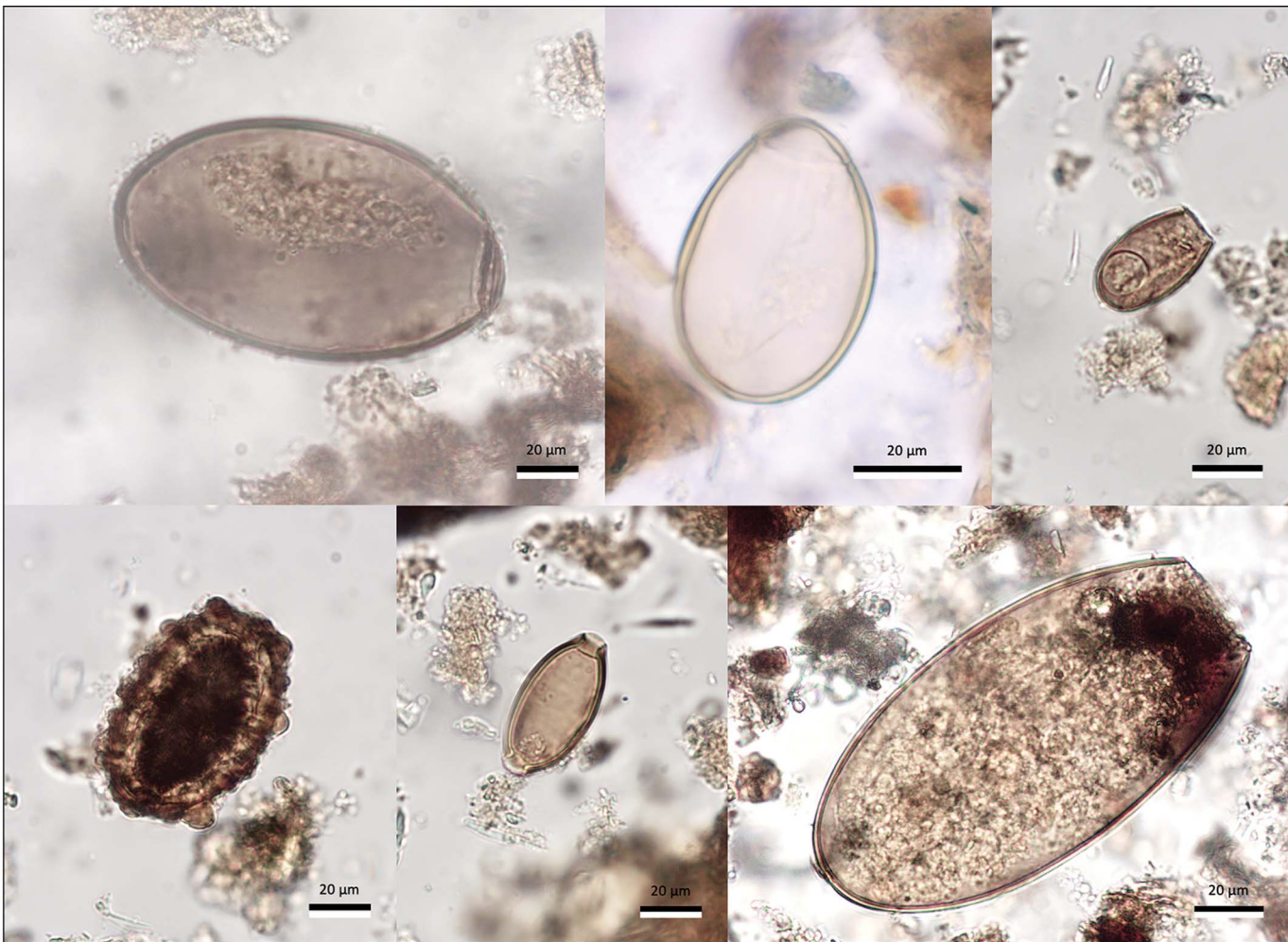
Figure 4. Parasite eggs from the Leiden cesspits. Top left: cf. Echinostoma sp. (dimensions 119 \times 72 \mu\text{m} ); top centre: Diphyllobothriidae ( 52 \times 36 \mu\text{m} ); top right: cf. Dicrocoelium sp. ( 36 \times 22 \mu\text{m} ); bottom left: roundworm ( 78 \times 48 \mu\text{m} ); bottom centre: whipworm ( 53 \times 26 \mu\text{m} ); bottom right: cf. Fasciola hepatica ( 141 \times 73 \mu\text{m} ) (figure by authors).
