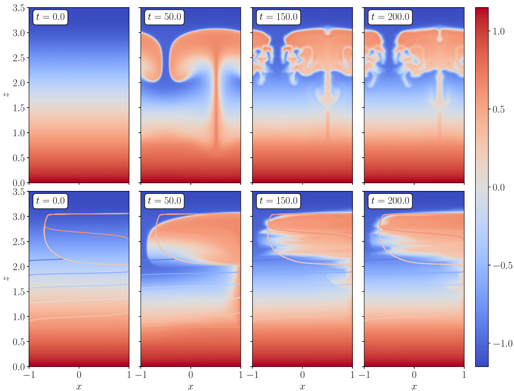
FIGURE 17. The relaxation of the equilibrium defined by (2.30) at \text{Re} \sim 10^2 . The initial velocity field is given by (4.5). Upper panels show the evolution of \ln(s/\chi) in x - z space. Lower panels show the same quantity but sorted horizontally at each z , with contours of the theoretical minimum-energy state (figure 7d) overlaid.
