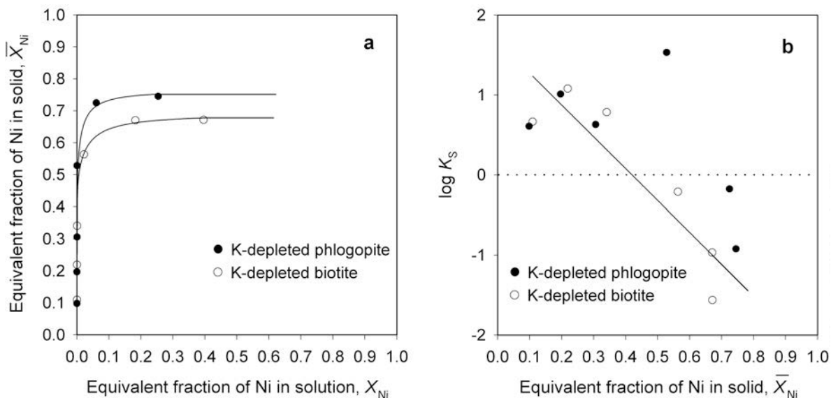
Figure 5. 2\text{Na}^+ \rightarrow \text{Ni}^{2+} ion exchange with K-depleted micas: (a) isotherms and (b) Kielland plots ( K_S = K_{\text{Na}}^{\text{Ni}} ).
