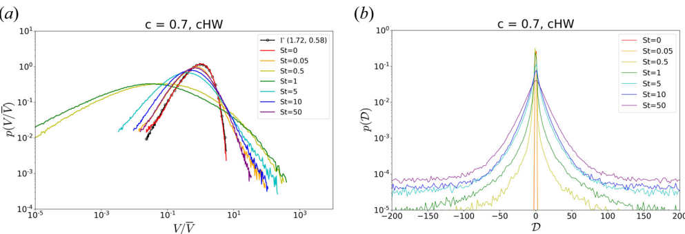
FIGURE 16. (a) PDF of volume normalised by the mean ( V/\bar{V} ) and (b) PDF of the impurity velocity divergence D for different Stokes numbers for ^{184}\text{W}^{44+} ( \alpha = 0.48 ) in the quasi-adiabatic regime ( c = 0.7 , cHW model).
