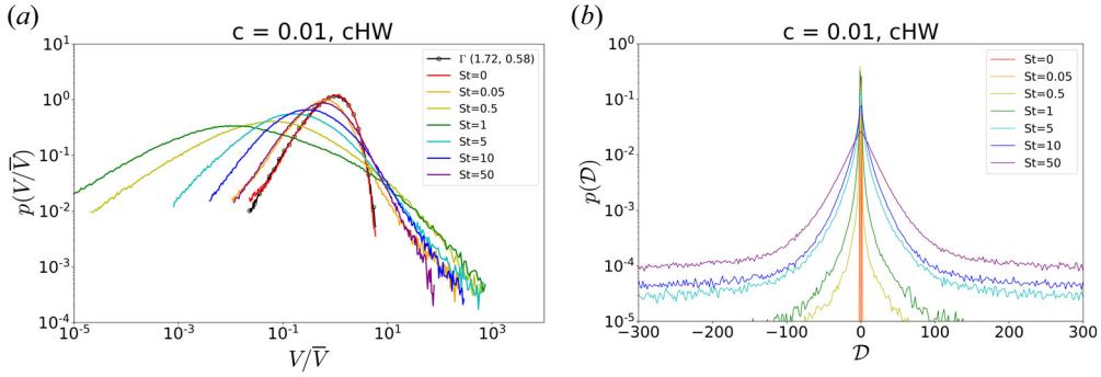
FIGURE 10. (a) PDF of volume normalised by the mean ( V/\bar{V} ) and (b) PDF of impurity velocity divergence \mathcal{D} for different Stokes numbers for ^{184}\text{W}^{20+} ( \alpha = 0.22 ) in hydrodynamic regime ( c = 0.01 , cHW model).
