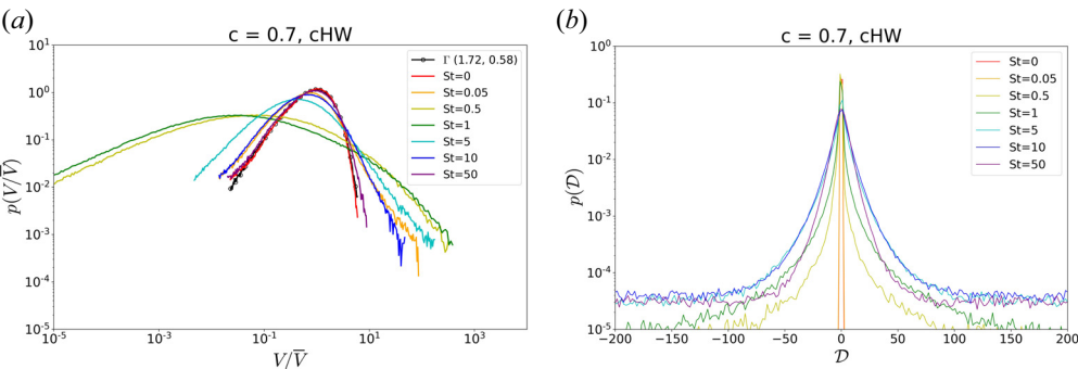
FIGURE 15. (a) PDF of volume normalised by the mean ( V/\bar{V} ) and (b) PDF of impurity velocity divergence D for different Stokes numbers for ^{184}\text{W}^{1+} ( \alpha = 0.01 ) in the quasi-adiabatic regime ( c = 0.7 , cHW model).
