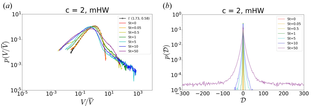
FIGURE 14. (a) PDF of volume normalised by the mean ( V/\bar{V} ) and (b) PDF of the impurity velocity divergence \mathcal{D} for different Stokes numbers for {}^{184}_{74}\text{W}^{20+} ( \alpha = 0.22 ) in zonal flows ( c = 2 , mHW model).
