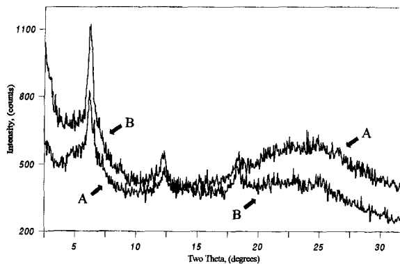
Figure 8. Increasing detection of clay peaks with decreasing glancing angle from 1.0^\circ (A) to 0.6^\circ (B) in GID analysis of a 0.010 \text{ mg cm}^{-2} Benndale sample.
