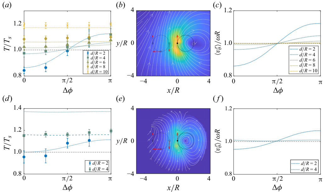
Figure 4. Hydrodynamic interactions between rotating helices under confinement ( a – c ) R_0 = 7R and ( d – f ) R_0 = 3.5R . ( a, d ) Torque on one helix in the helical pair as a function of phase difference \Delta\phi at different spacings d . Symbols denote experimental data, while dotted lines represent model predictions (3.2). The green dashed line in ( d ) is the model prediction using experimentally obtained T_e/T_c , instead of (3.1). ( b, e ) Flow field in the x – y plane of a rotating helix positioned at (R, 0) . The circle on the right indicates the helix's trajectory, while the dashed circle on the left represents the trajectory of an imaginary helix. Three phase differences between the real helix and the imaginary helix are shown, consistent with those in figure 3( a ). ( c, f ) Velocity of the imaginary helix in the reference frame of local flow, \langle v_\theta^r \rangle , normalised by the helix's rotation speed in the lab frame, \omega R , as a function of \Delta\phi at different d .
