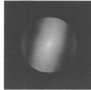
Fig. 2. Power spectrum of the triple system HIP 7372 ABC.
