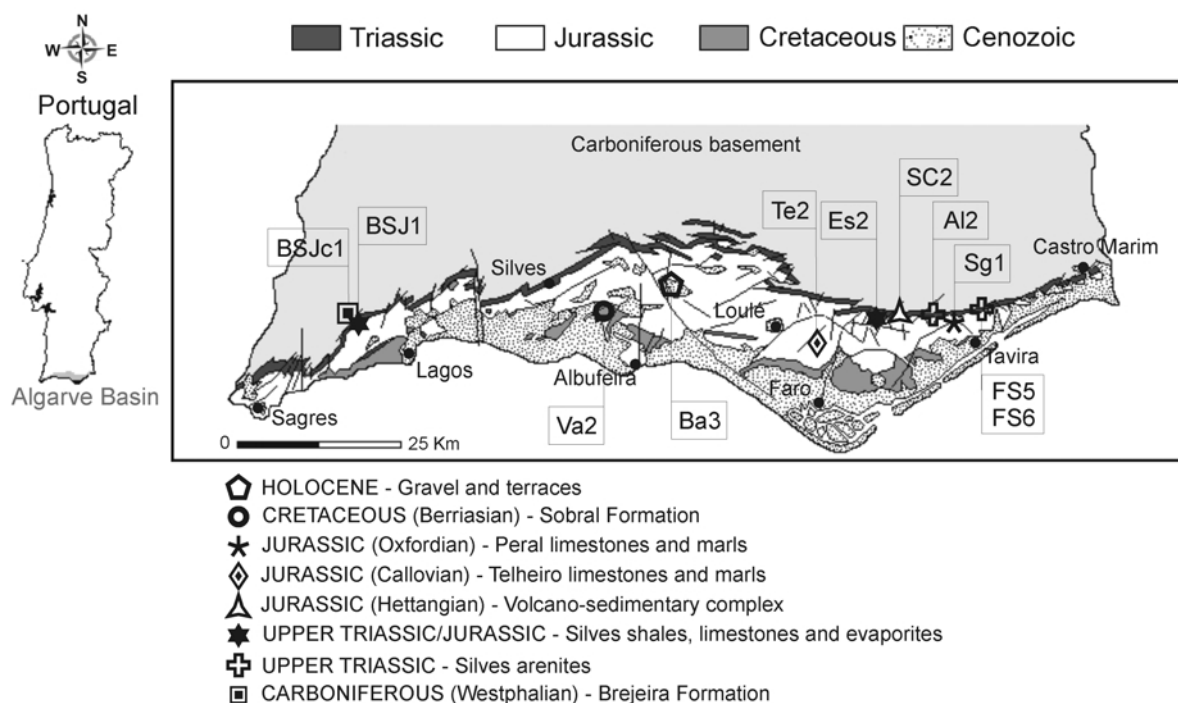
Figure 1. Simplified geologic map of the Algarve Basin showing sample locations.
