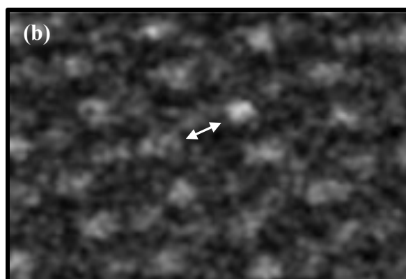
Figure 3: Two consecutive 2-frame images from Figure 1 showing neighboring Ti-O columns that fluctuate in intensity between (a) and (b). Intensity fluctuations may be attributed to shot noise, or to structural reconfigurations from defects present in the anatase structure.
