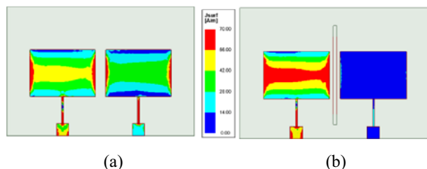
Figure 10. Current distributions on patches at resonances (a) without and (b) with the proposed wall.
