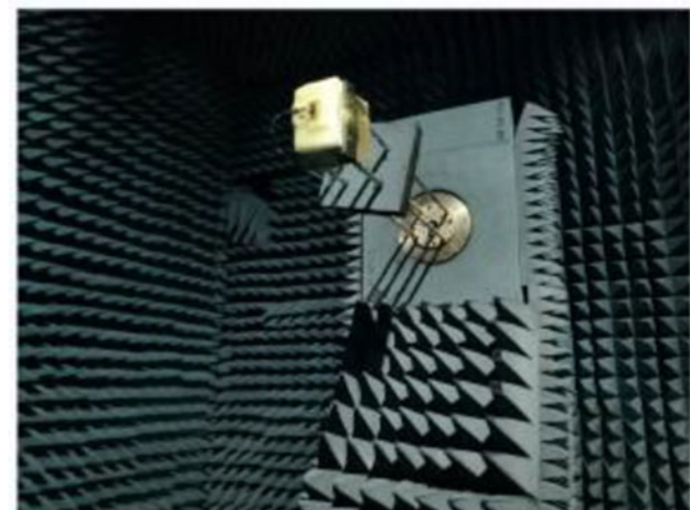
Figure 3. Measurement in an anechoic chamber.
