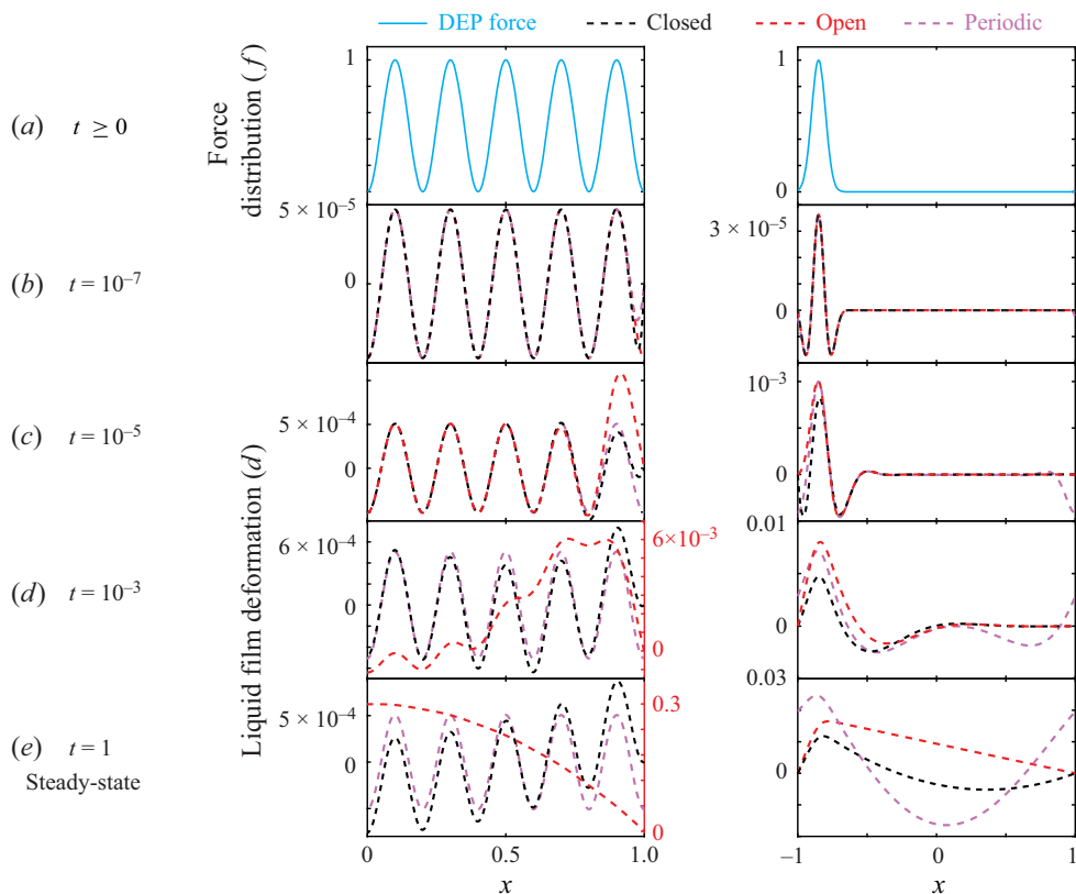
Figure 2. The effect of different sets of boundary conditions (BCs) on the film dynamics for harmonic (left column, l ) and localized (right column, r ) force distributions. (a) The external force distributions applied on the liquid-air interface along the chamber. (b–e) Comparison of the analytical solutions for the case of pinned film and impermeable boundaries (‘Closed chamber’, black dashed line), pinned film and permeable boundaries (‘Open chamber’, red dashed line) and ‘Periodic’ (light purple dashed line), at different times. All panels in the left column present half of the chamber, with a symmetry line at x=0 . At early times, the deformation exhibited by all systems is nearly identical. With time, deviations start evolving from the boundaries inward. At the harmonic forcing case, since the force is strictly positive, the Open system results in a continuous influx of liquid which ultimately leads to inflation of the interface to a ‘balloon’-like structure. In contrast, the Closed and the Periodic systems, owing to their fixed mass, maintain short-wave deformations which follow the force distribution even at steady state, as shown in (e.l). The film deformation of the Open system at late times is much larger than the deformation of the other two systems. Thus, (d.l) and (e.l) present two different y axes, left for Closed and Periodic systems, and right for the Open system. In the Gaussian forcing case the Open and the Closed systems show similar behaviour due to the pinning condition (although the latter is not a fixed-volume system) in contrast to the Periodic system. The solution presented for all systems is for the case of an initially flat interface, d_0(x) = 0 and Bo = 0 .
