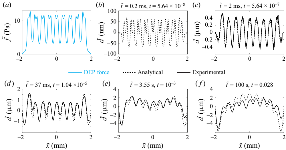
Figure 5. Validation of the analytical model against experimental measurements. (a) The DEP force distribution at the oil-air interface resulting from an array of parallel electrodes, as obtained from an electrostatic calculation in accordance with Gabay et al. (2021). (b–f) The evolution of the film deformation from early times to steady state, showing the dominance of high wavenumbers at short times, and the gradual appearance of small wavenumbers with time. The analytical model successfully captures both the local and the global behaviour of the film across multiple time scales. The chamber length is 4 mm, and is thus slightly truncated on the right by the 3.8 mm field of view of the holographic microscope. In this experiment we use silicone oil with kinematic viscosity of 200 cSt. The rest of the parameters (liquid properties and electric voltage actuation) are listed in the § 5.1.
