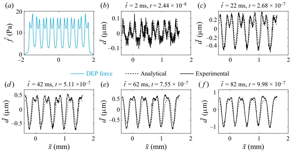
Figure 6. Validation of the analytical model with experimental measurements at very small non-dimensional times, t < 10^{-6} . (a) The DEP force distribution at the oil–air interface of a 30 \mu\text{m} film, as obtained from electrostatic calculations (Gabay et al. 2021). (b–f) Comparison between the analytical solution (black dashed line) and the experimental measurements (black solid line) of the film deformations at different times. At short times the ‘tooth’-shaped peaks, corresponding to the highest spatial frequency, dominate the deformation. At later times, additional lower frequencies appear and overtake the higher frequencies in amplitude. In this experiment we use silicone oil with kinematic viscosity of 1000 cSt. The rest of the parameters (liquid properties and electric voltage actuation) are listed in § 5.1.
