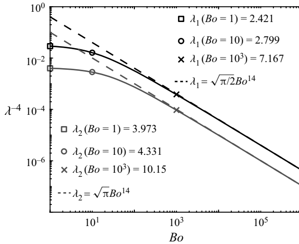
Figure 3. The eigenvalues of the system as a function of the Bond number. The response time of the system is proportional to \lambda^{-4} , which for large Bo is inversely proportional to Bo . Thus, as Bo increases, e.g. by increasing the density of the liquid or increasing the size of the container, the response time of the system can shorten significantly.
