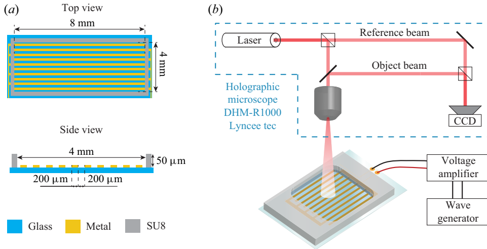
Figure 4. Illustration of the fluidic chamber the experimental set-up. (a) The resulted fluidic chamber configuration and it's fabrication process. At first, the electrodes are created by a lift-off process using a 2 nm thick Pt layer sandwiched between two 2 nm thick Ti layers on a borosilicate wafer which forms an array of interdigitated electrode configuration with 200 \mu\text{m} wide electrodes, gapped by 200 \mu\text{m} edge to edge. Second, the chamber's walls are created by patterning a 50 \mu\text{m} thick layer of SU-8 photoresist on top of the wafer. Finally, we diced the wafer to separate individual devices. (b) Schematic illustration of the experimental set-up. The device is mounted on a home-made connector composed of 3D printed housing and a printed circuit board (PCB) containing electric pins interfacing the device with a voltage amplifier (2210-CE, TREK), which amplifies the voltage output of a wave generator (TG5012A, AIM-TTI Instruments). The device is placed under a digital holographic microscope (DHM R1000, Lyncee tec) allowing observation of the oil-air interface by recording a hologram image on a digital sensor and using a numerical algorithm for real-time reconstruction.
