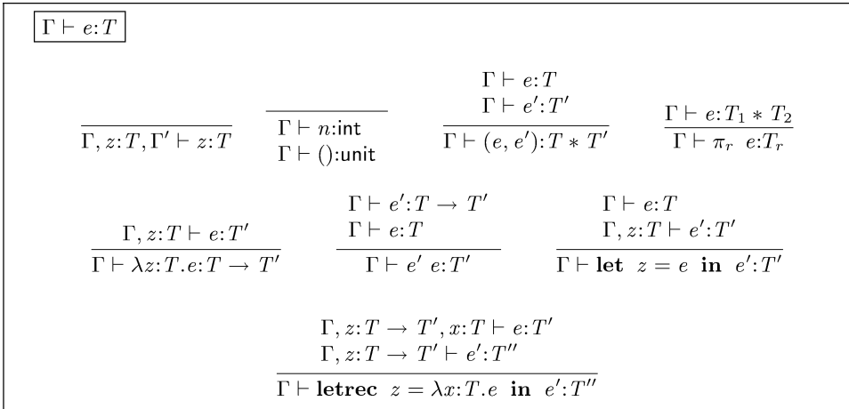
Fig. 1. Lambda calculi—typing.
