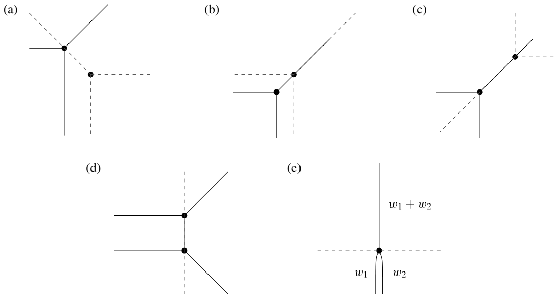
FIGURE 4. Pretangent morphisms.
