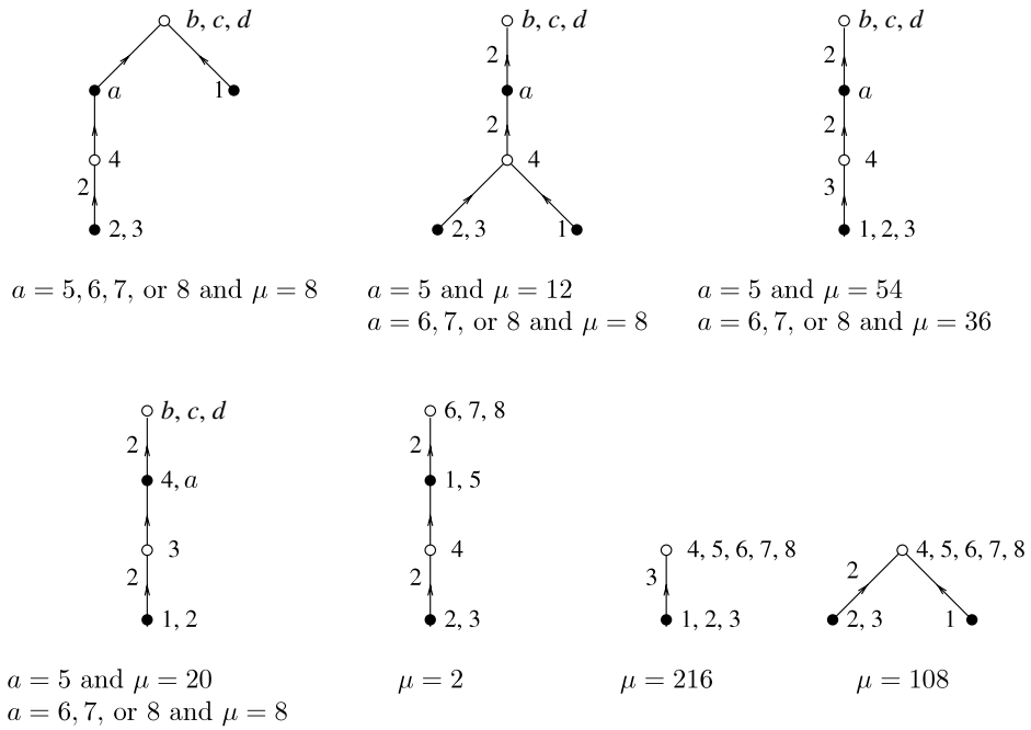
FIGURE 21. Computation of N_{3,0}(1; 1^7) = 600 with \mathcal{L}^{\text{comb}} = \{2, \dots, 8\} .
