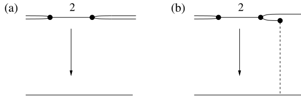
FIGURE 2. Example of tropical morphisms f : C \rightarrow \mathbb{R} .
