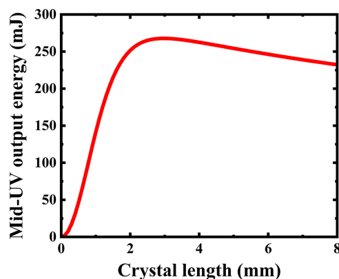
Figure 2. Calculated mid-UV output energy at 266 nm versus BBO crystal length under a 700 mJ, 532 nm pump with beam radius of 10 mm.
