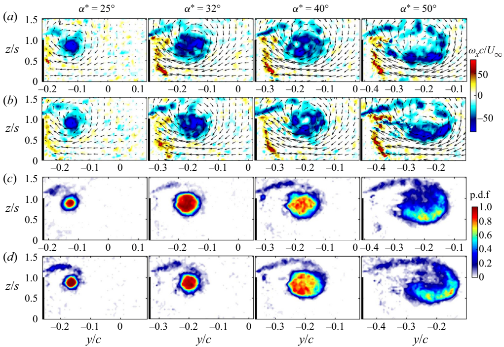
Figure 12. Distribution of instantaneous flow fields in the y - z plane at the pivot ( x_m/c = 0.52 ). The vorticity fields at K = 0.01 (a), the vorticity fields at K = 0.08 (b), probability density function of the number of TV vortices identified by the \lambda_2 -criterion at K = 0.01 (c) and at K = 0.08 (d).
