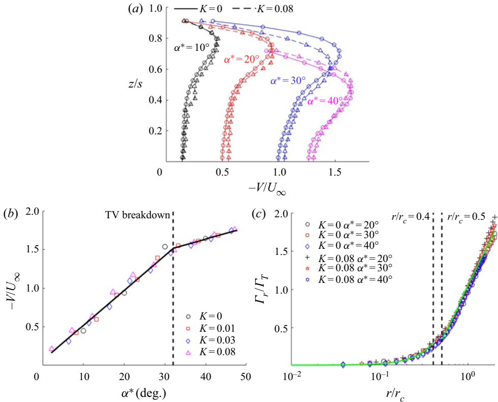
Figure 14. (a) The V -component velocity profiles over the suction side of the wing from the TV centroid to the mid-span at the pivot at K = 0 and K = 0.08 , (b) the peak velocity of V between the TV centroid and the mid-span as a function of \alpha^* at different pitch rates, (c) non-dimensional circulation vs its radius at different AoAs at the pivot.
