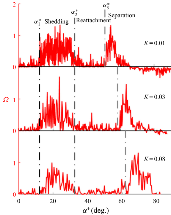
Figure 20. Non-dimensional vorticity flux \Omega at the mid-span vs \alpha^* when the wing is pitching at K = 0.01, 0.03 and 0.08 .
