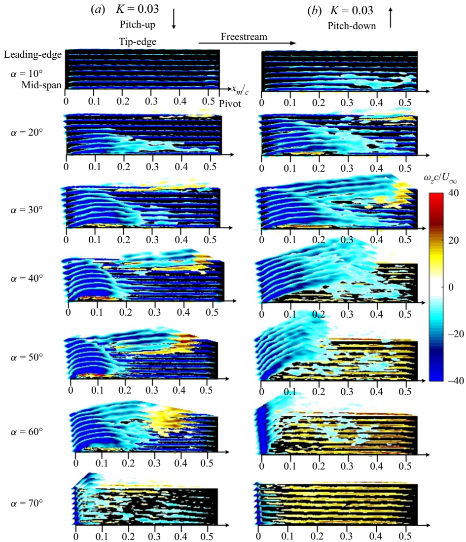
Figure 17. The phase-averaged normalized spanwise vorticity ( \omega_z c/U_\infty ) along the span vs AoA for the pitch-up and pitch-down wing at K = 0.03 . The colour bar on the right side applies to all plots.
