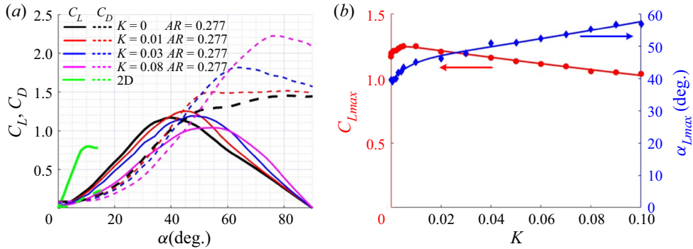
Figure 4. The aerodynamic characteristics of a very low AR flat-plate wing as a function of AoA and the pitch rate: (a) the lift coefficient C_L and the drag coefficient C_D as compared with those of a stationary 2-D thin flat plate ( Re = 10^5 ) by Pelletier & Mueller (2000); (b) the maximum lift coefficient C_{Lmax} and the maximum lift angle \alpha_{Lmax} .
