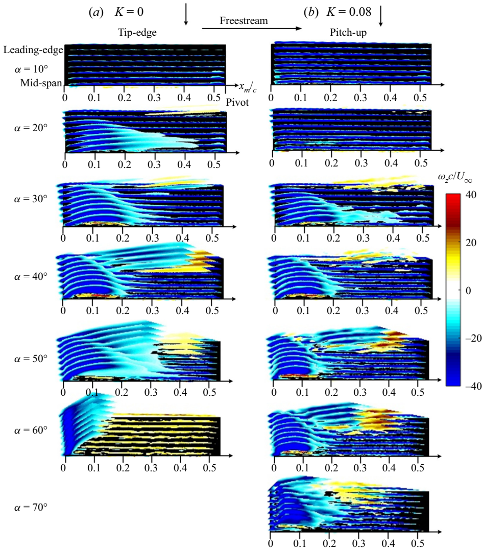
Figure 16. The phase-averaged normalised spanwise vorticity ( \omega_z c/U_\infty ) along the span vs AoA for the baseline case and the wing pitching at K = 0.08 . The colour bar on the right side applies to all plots.
