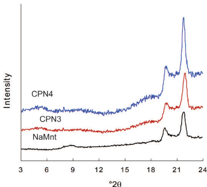
Figure 3. XRD patterns of NaMnt, clay-polymer nanocomposite 3 (CPN3), and clay-polymer nanocomposite 4 (CPN4) treated with perbromide reagent.
