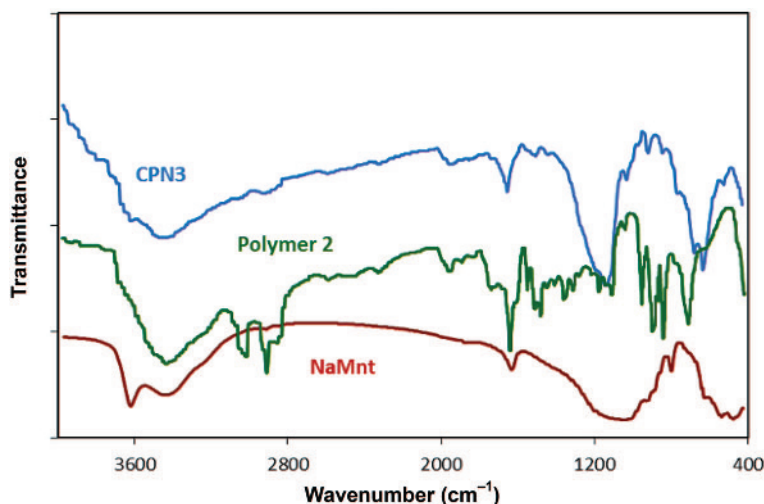
Figure 2. IR spectra of NaMnt, linear polymer 2, and CPN3.
