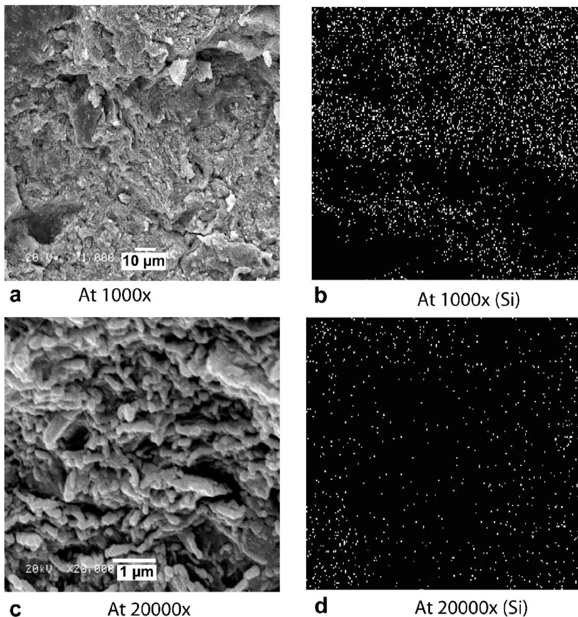
Figure 5. SEM images (a,c) with X-ray mapping (b,d) of CPN3.
