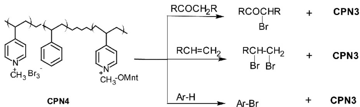
Figure 7. Bromination with reagent CPN4.
