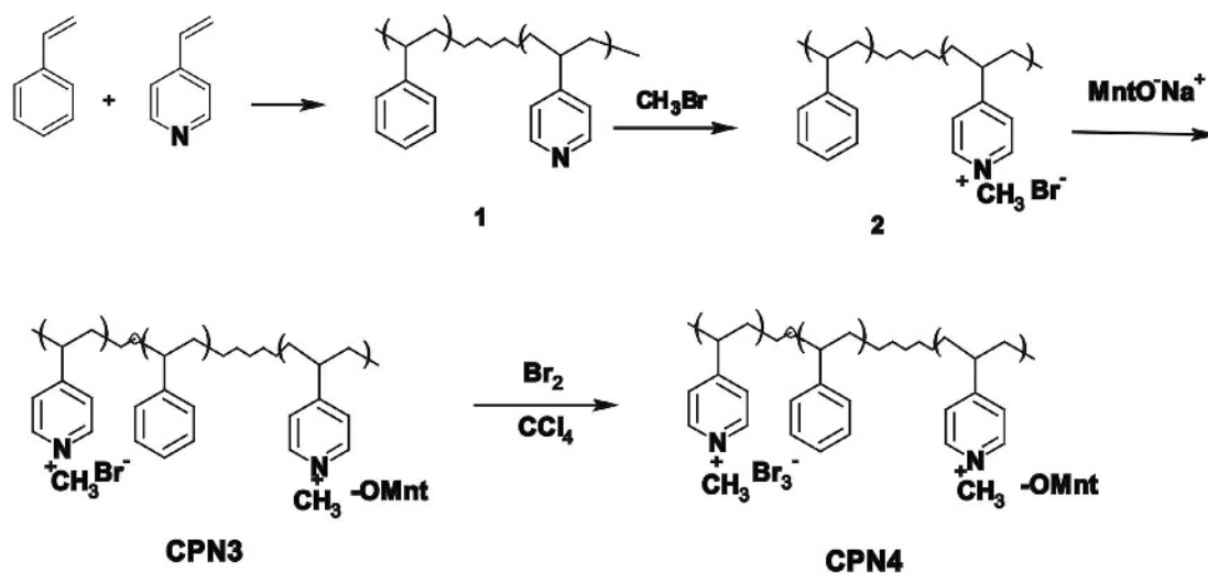
Figure 1. Synthesis of brominating reagent CPN4.
