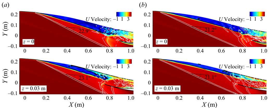
Figure 22. Contours of the instantaneous streamwise velocity for slice z = 0 mm and z = 30 mm at (a) t u_{\infty} / L = 3006.8 and (b) t u_{\infty} / L = 3228.9 . The black solid line denotes the isoline of u = 0 and the white solid line signifies the isoline of \partial P / \partial X = 25 .
