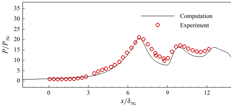
Figure 6. Experimental and computed wall pressure at the centre line of the double-fin configuration.
