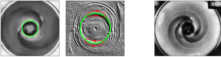
Fig. 3. Top: left: interarm anticyclonic vortices in the zone of the generating shear on the corotation radius, forming a single whole with the spiral waves. Right: branching of arms in an intermediate spiral structure at a stage of the transition from mode four to mode two caused by a slow increase in rotation velocity of the core.
