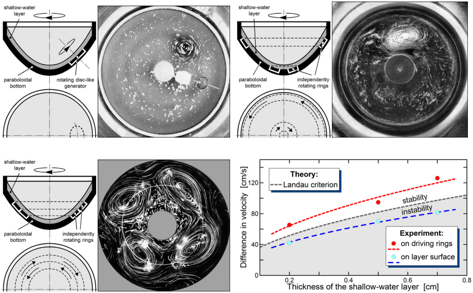
Fig. 1. Top: anticyclonic Rossby vortex drifting free and counter to the “global” rotation from the place of its impulse generation ( left ); Rossby autosoliton an anticyclone generated constantly by an anticyclonic shear between distant counter flows ( right ). Bottom: chain of cyclones generated by an instability of a cyclonic shear between adjacent counter flows and difference in velocities at the upper threshold of the instability of the cyclonic shear versus thickness of the layer (the Landau criterion for the threshold difference is presented as 2\sqrt{2g^*H} ).
