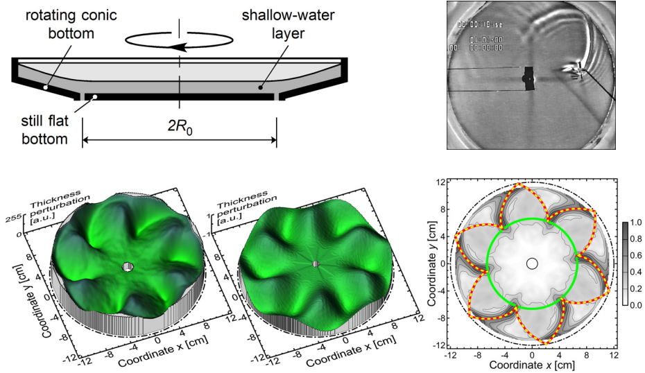
Fig. 4. Left: schematic of the experimental setup for studying the over-reflection instability and thickness perturbation in unstable mode six as experimental (below left) and theoretical (below right) results. Right: waves from a body revolving in the layer with their reflections from a circular wall and magnitude of the thickness gradient in the wave structure (experiment) overlaid with a resonantly multi-reflected shock front (theory).
