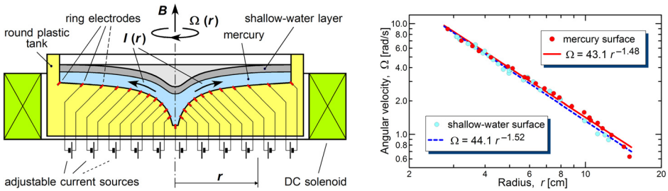
Fig. 5. Left: schematic of a setup with smooth differential rotation of a shallow-water layer by means of underlying MHD-driven mercury. Right: Keplerian rotation realised in shallow water over the MHD-driven mercury ‘bottom’ (shallow-water layer is about 0.5 cm thick).
