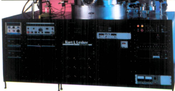
Supersystem III vacuum system with substrate entry lock
