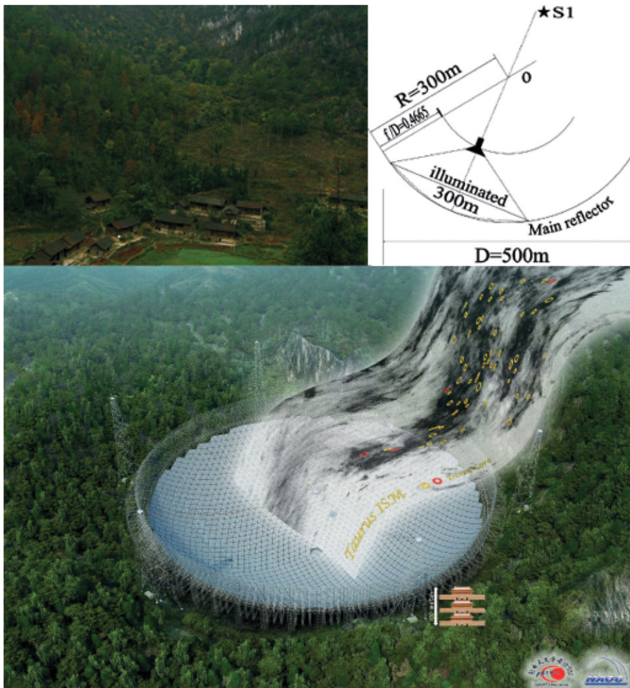
Figure 1. Upper Left: Partial view of the original site as seen in Nov of 2009. Upper Right: FAST optical geometry. Lower: A 3D model of FAST.
