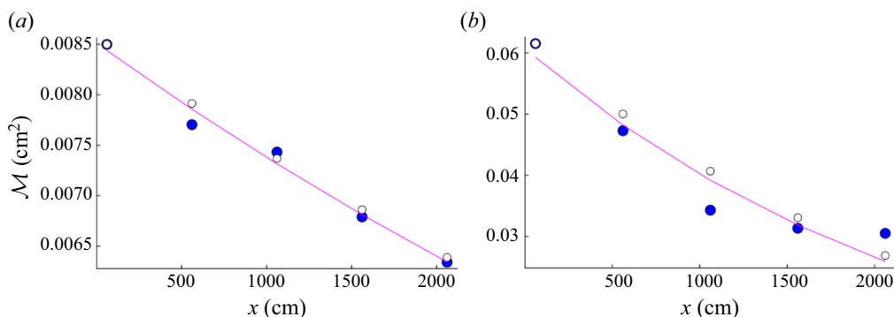
Figure 8. Plots of \mathcal{M} versus x for the Hammack & Segur (1978) experiments with (a) A_0 = 0.5 cm and (b) A_0 = 1.5 cm. The blue dots represent the experimental measurements, the magenta curves represent the best-fit exponentials of the experimental data and the black circles represent the dsWhitham predictions.
