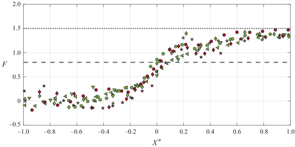
Figure 6. Pressure evolution across separation represented through the coefficient of free interaction (for symbols, see table 3; dashed black line corresponds to F_s = 0.8 , and dotted black line corresponds to F_p = 1.5 ).
