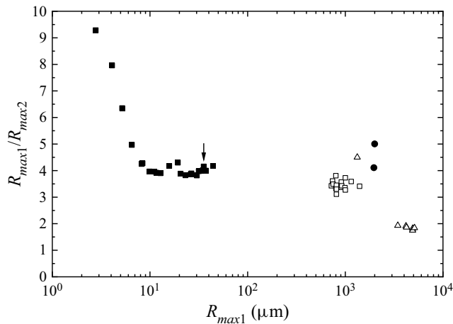
Figure 15. Ratio R_{max1}/R_{max2} under ambient conditions as a function of maximum bubble radius. ■ Present study; \triangle Vogel & Lauterborn (1988); \square Akhatov et al. (2001); \bullet Sinibaldi et al. (2019). The ratio is a measure of energy dissipation during the first collapse. Since most energy is carried away by acoustic radiation, it is also indicative of the amplitude of the collapse pressure. An arrow marks the data point corresponding to the signal of figure 6. The collapse of the highly spherical laser-induced bubbles investigated in this paper is more vigorous than that of larger, millimetre-sized bubbles, where usually smaller focusing angles were used for plasma generation and a combination of elongated plasma shape and buoyancy led to deviations from spherical shape. The largest R_{max1}/R_{max2} value for millimetre-sized bubbles was observed by Sinibaldi et al. (2019) for tight focusing at NA = 0.6. The R_{max1}/R_{max2} ratio increases for R_{max1} < 10 \mu\text{m} , where surface tension and viscosity become important.
