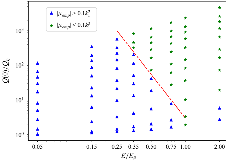
Figure 9. Phase diagram of the runs in the parametric space of the energy level E/E_\# and the initial enstrophy Q(0)/Q_\eta (both in log scales). Markers \blacktriangle (blue) and \star (olive green) denote the runs with \mu_{emp} larger and smaller than 0.1k_1^2 , respectively. The red dashed line roughly delineates the regimes of non-uniform and homogeneous background PV in the low-energy region of E < E_\# .
