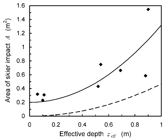
Fig. 12. Area of skier influence A (where \sigma_z(x, y) > \sigma_z(x = 0, y = 0)/\sqrt{2} ) vs effective depth z_{eff} determined from all experiments for which w and L are known. Solid line is quadratic fit to data. Dashed line shows point load model (three-dimensional) for reference.
