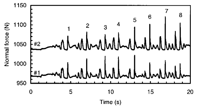
Fig. 7. Normal forces due to jumping measured in the snow cover on two load cells 0.1 m apart ( z_{\text{eff}} = 0.92 m). Lower curve for load cell 1, upper curve for load cell 2. The first four jumps are on load cell 1. Jump No. 5 is in between load cells 1 and 2. The last three jumps (6–8) are on load cell 2.
