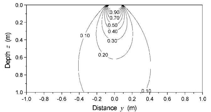
Fig. 4. Contour plot of normal stress (normalized to surface stress q ) below a skier vs depth z in transversal section ( y-z plane), perpendicular to axis of skis ( x ). Skier load modelled as strip load ( w_0 = 0.2 m).
