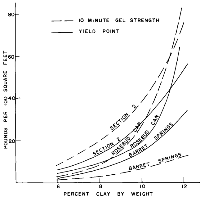
Fig. 5. Variations of yield point and 10-min gel strength with percentage of montmorillonite in clay-water mixtures for three Nevada samples.
