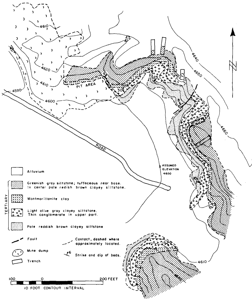
Fig. 2. Geologic map of the Rosebud Canyon montmorillonite deposit, Pershing County, Nevada.
