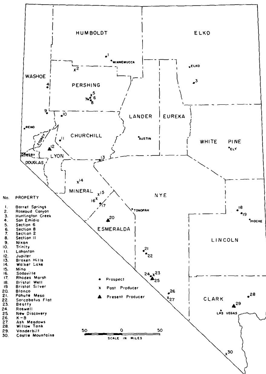
Fig. 1. Map showing montmorillonite deposits in Nevada.
