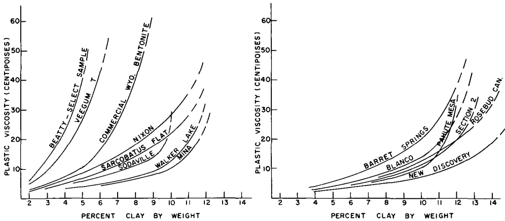
Fig. 4. Variations of plastic viscosity with percentage of montmorillonite in clay-water mixtures for fourteen samples.
