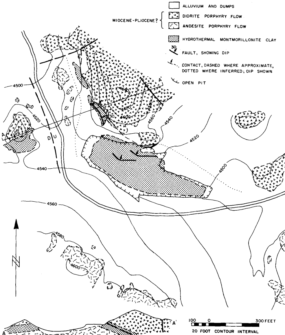
Fig. 3. Geologic map and cross section of the Jupiter montmorillonite deposit, Lyon County, Nevada.
