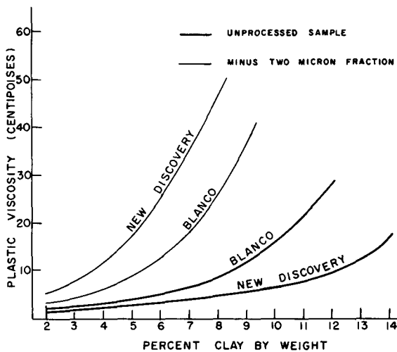
Fig. 6. Variations of plastic viscosity with percentage of solids in clay-water mixtures for unprocessed samples and the -2\mu fractions.
