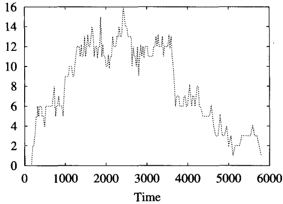
Fig. 2. The number of stable hierarchical systems in model 1.
