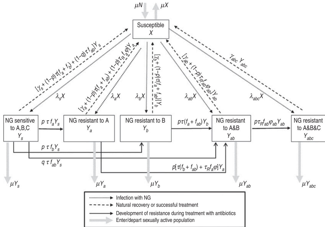
Fig. 1. Flow diagram of the model for the transmission of Neisseria gonorrhoeae (NG). Infected individuals are distinguished according to whether they are infected with a strain of NG sensitive to antibiotics A, B, and C ( Y_s ); resistant to antibiotic A only ( Y_a ); resistant to antibiotic B only ( Y_b ); resistant to antibiotics A and B ( Y_{ab} ); or resistant to antibiotics A, B, and C ( Y_{abc} ). Model parameters are defined in Table 1.
