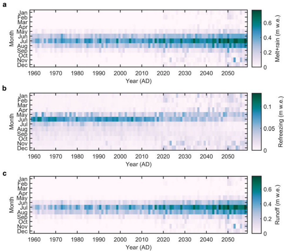
Fig. 8. Diagrams showing monthly melt and rain (a), refreezing (b) and runoff (c) for the RCP 4.5 scenario and averaged for the entire land area of Svalbard.
