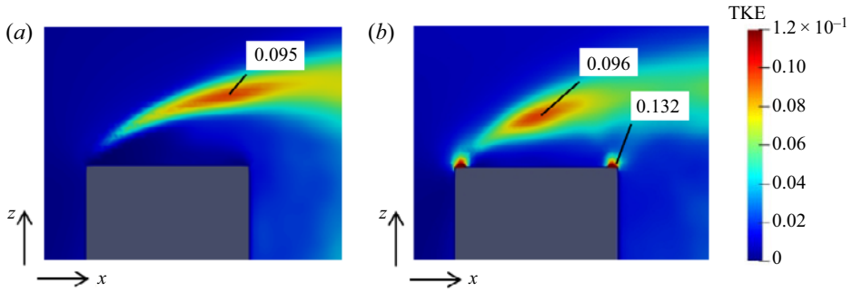
Figure 7. The TKE distribution near the top surface at y = 0 for an oncoming wind angle of \alpha = 0^\circ . (a) The unforced case, (b) the controlled case of St_f = 1.5 . Local maxima in the TKE are marked as values in the plots.
