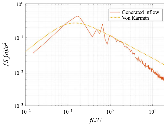
Figure 21. Comparison of PSD in the flow direction with the von Kármán spectrum at the model building height.
