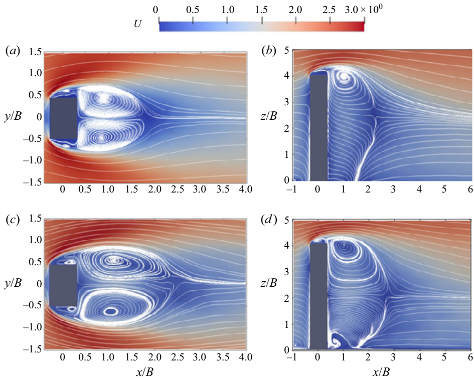
Figure 5. Time-averaged streamwise velocity field and projected streamlines for an oncoming wind angle of \alpha = 0^\circ . The unforced case: (a) top view in the horizontal plane z = 0.5H , (b) side view in the symmetry plane y = 0 . The controlled case of St_f = 1.5 : (c) top view in the horizontal plane z = 0.5H , (d) side view in the symmetry plane y = 0 .
