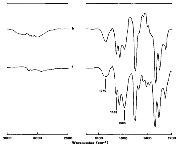
Figure 3. Infrared differential spectra of Fluzifop-treated homoionic clays: (a) Cu and (b) Cu after \text{CHCl}_3 washing.
