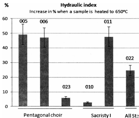
Figure 2 Test of solubility in standard HI determination. Percent increase of the HI of a sample aliquot after heating it to 650 °C compared with an unheated aliquot of the same sample powder.
