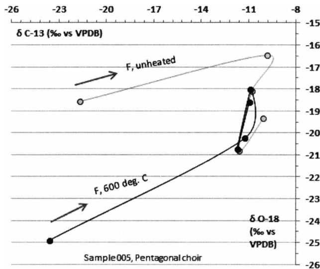
Figure 14 \delta^{13}\text{C} vs. \delta^{18}\text{O} for 5 \text{CO}_2 fractions for an unheated sample aliquot and a heated aliquot (600 °C).
