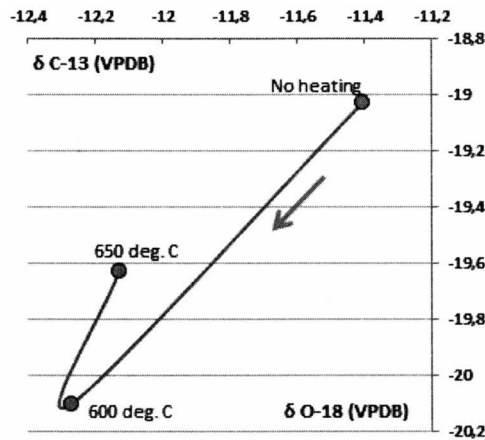
Figure 12 δ 13 C and δ 18 O trends when the powder of sample TTK 005 was heated at 600 °C and 650 °C, respectively.
