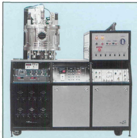
"Supersystem" with 3 Torus® guns
