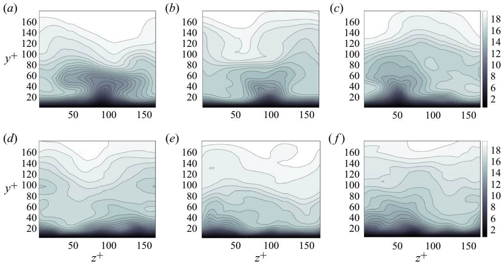
Figure 26. Examples of base flows able to support turbulence (a–c) and unable to support turbulence (d–f) from cases NF-TG180 i discussed in § 6.3. Visual inspection of the base flows suggests that spanwise variations of U are crucial to sustain turbulence.
