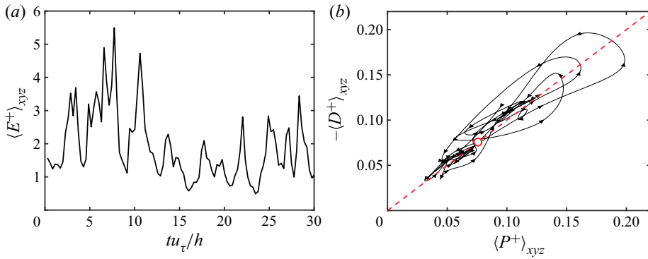
Figure 15. (a) The history of the domain-averaged turbulent kinetic energy of the fluctuations \langle E \rangle_{xyz} . Note that only 30h/u_\tau units of time are shown in the panel, but the simulation was carried out for more than 300h/u_\tau . (b) Projection of the flow trajectory onto the average production rate \langle P \rangle_{xyz} and dissipation rate \langle D \rangle_{xyz} plane. The arrows indicate the time direction of the trajectory, which on average rotates counterclockwise. The red dashed line is \langle P \rangle_{xyz} = -\langle D \rangle_{xyz} and the red circle \langle P \rangle_{xyz} = -\langle D \rangle_{xyz} . The trajectory projected covers 15h/u_\tau units of time. Results are for the channel with suppressed modal instabilities NF-SEI180.
