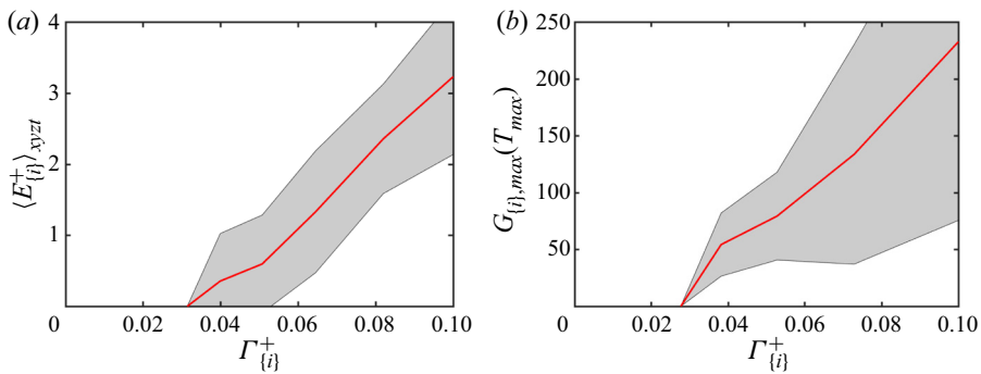
Figure 25. (a) Mean turbulent kinetic energy and (b) maximum gain G_{[i],max} at T = T_{max} conditioned to the marker for the spanwise-shear strength \Gamma_{[i]}^+ = \langle (\partial U_0(y, z, t_i) / \partial z)^2 \rangle_{yzt}^{1/2} compiled over NF-TG180 i . The red solid line represents the mean value; the shaded area denotes \pm one standard deviation.
