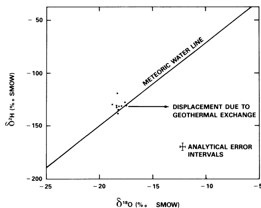
Fig 4. \delta^2\text{H} vs \delta^{18}\text{O} of the 10 waters reported, showing no displacement due to geothermal exchange
