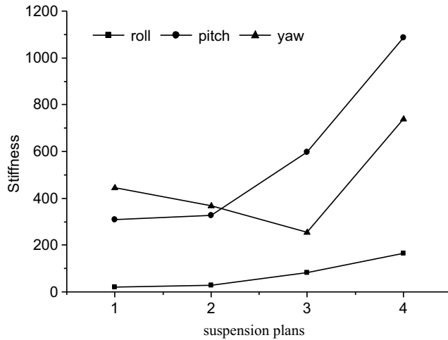
Figure 12. Comparison of rotational stiffness for different suspension schemes.
