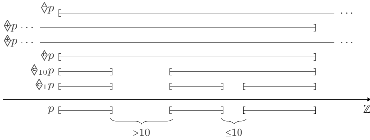
Fig. 1. The resulting intervals of the induced functions of the diamond operators when applied to the intervals at which p holds (denoted below the timeline). While \diamond closes all gaps, \diamond_{10} does not close the first gap, since it is greater than 10 time units.
