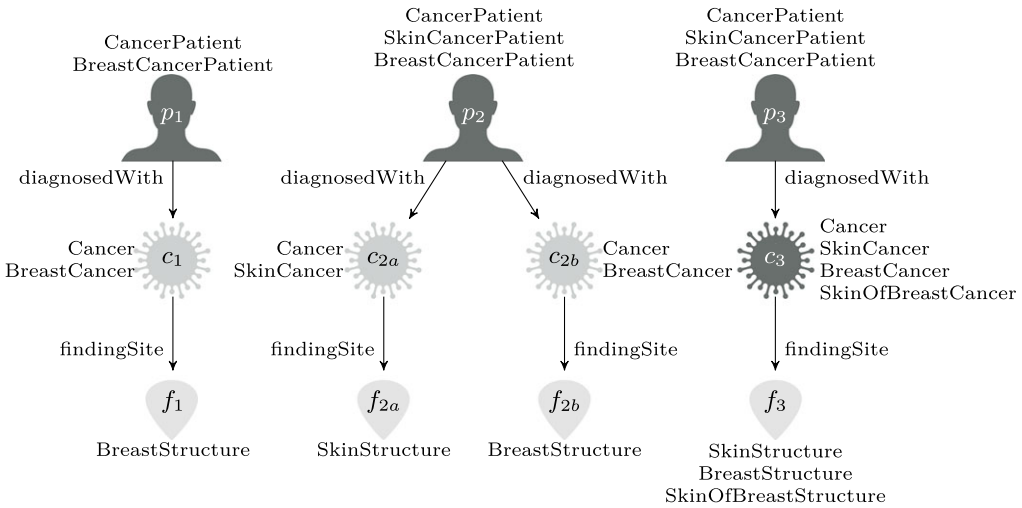
Fig. 2. The minimal canonical model \mathcal{I}_{\mathcal{K}_C} . The named individuals p_1, p_2, p_3 , and c_3 are depicted by dark grey figures, the remaining anonymous objects by light grey.
