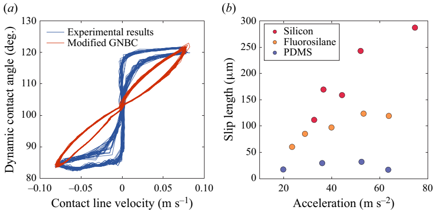
Figure 10. (a) Comparison between the angle–velocity relation obtained from experiment and predicted by modified GNBC. (b) Slip lengths extracted according to the modified GNBC for various substrates and accelerations.
